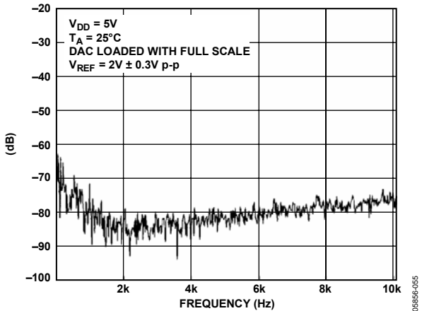
Figure 47. Total Harmonic Distortion
