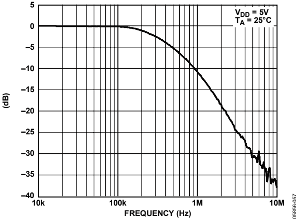
Figure 49. Multiplying Bandwidth
