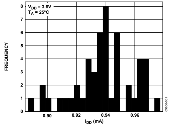
Figure 32. I_{DD} Histogram with Internal Reference, V_{REFOUT} = 1.25 V
